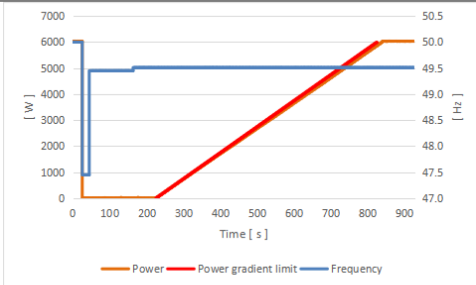
Graph_49.5Hz setting
