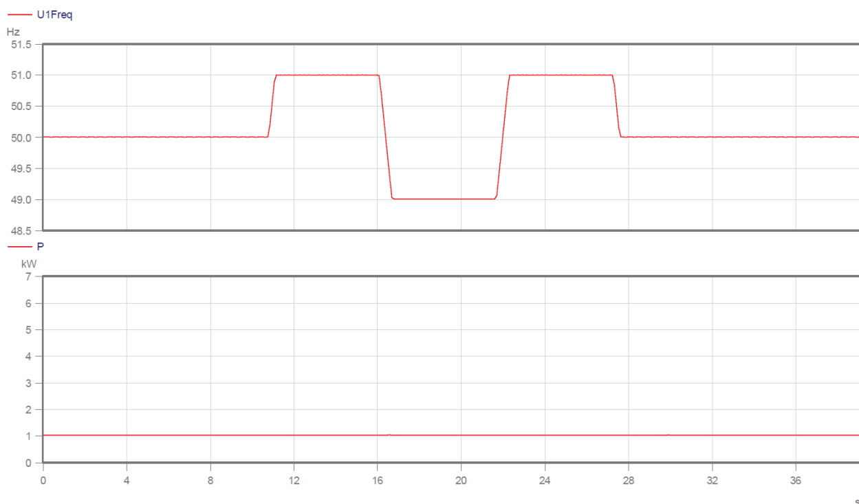
Figure 5-2 RoCoF withstand test results, showing grid frequency (upper plot) and output power (lower plot) for AFORE AF1K-SL-1 /1/
