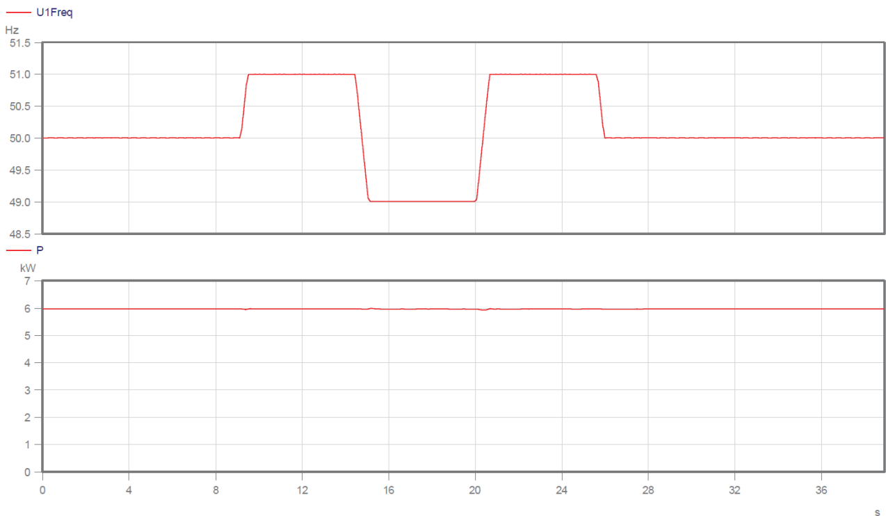
Figure 5-1 RoCoF withstand test results, showing grid frequency (upper plot) and output power (lower plot) for AFORE AF6K-SL /1/
